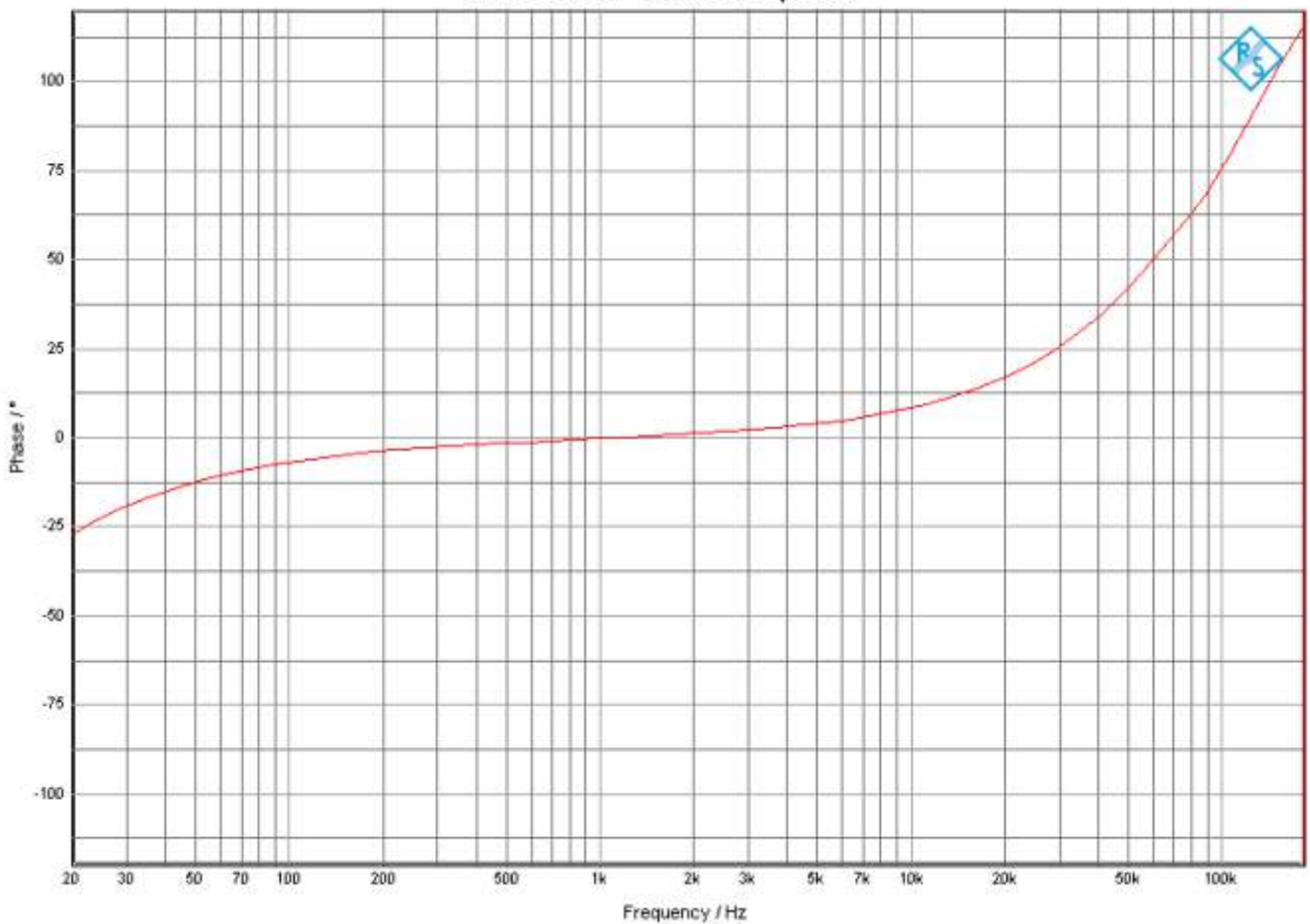
30SE3K0H - Phase response
