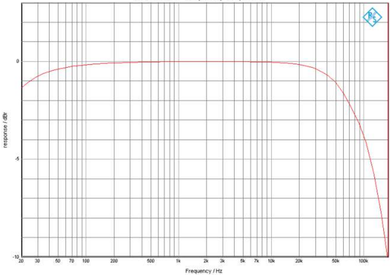
30SE3K0H - frequency response
